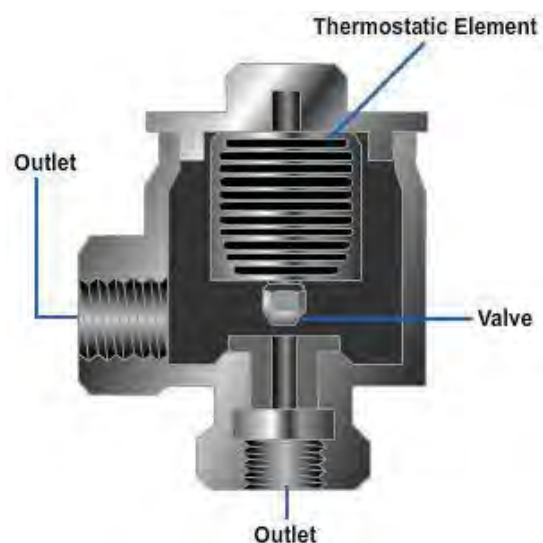
Figure 10-13 – Thermostatic trap.
