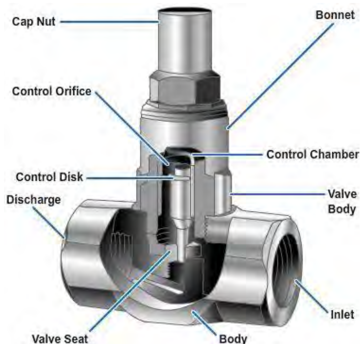
Figure 10-15 — Impulse trap.
