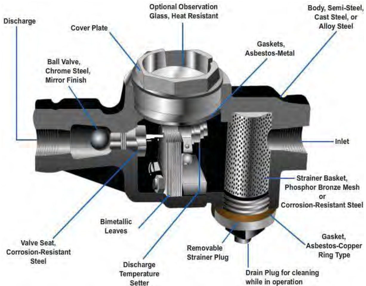
Figure 10-18-Bimetallic-element steam trap.
