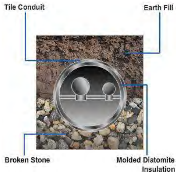
Figure 10-1 – One type of steam distribution conduit.
